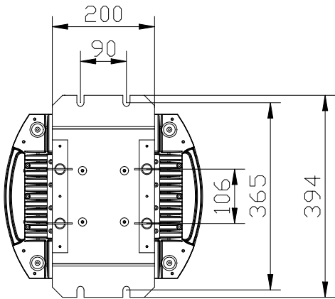
Base installation and its sizes: (unit: mm)
