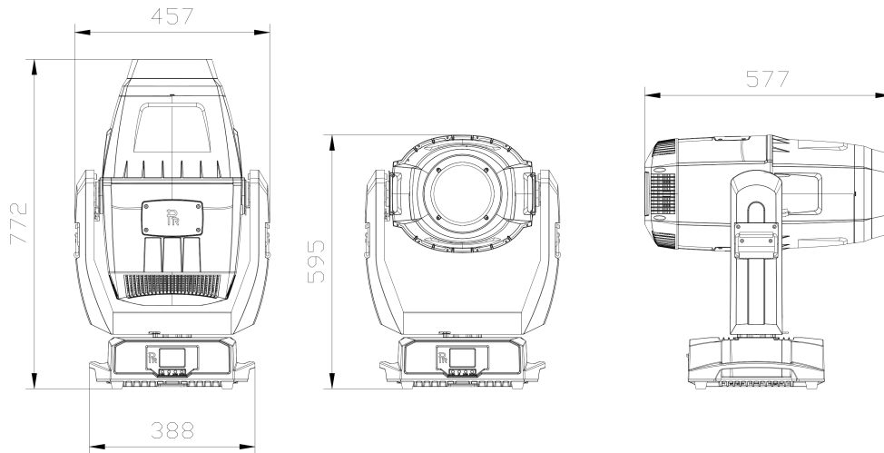
Base installation and its sizes: (unit: mm)
